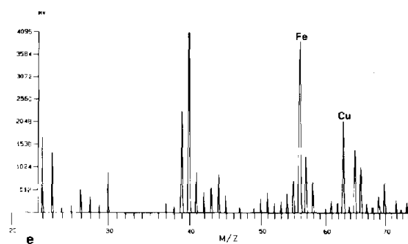
Figure 1. Partial mass spectra from various samples probed by LAMMA. Positive ion spectra show major peaks identified by their mass to charge ratios ( m/z ) where they are assumed to have a unit positive charge. Ordinate gives peak height rather than integrated peak intensity. Na 23; Mg 24; Al 27; P 30; S 32; K 39; Ca 40; Fe 56; Cu 63. (a) Cytoplasm of a Gaucher cell showing a high iron-related peak ( m/z = 56 ). (b) Genetic haemochromatosis, prior to phlebotomies; siderosomes in hepatocytes. (c) Same sample as (b), but the probed cell was a Kupffer cell; note that the iron-related peak is much lower than that of hepatocytic siderosomes. (d) Thalassaemia major, liver biopsy of a 3 month old infant showing an extremely high iron signal (saturated peak), as well as a significant aluminium peak ( m/z = 27 ). (e) Wilson's disease, patient 1. Probing of connective tissue cells from the pre-transplant cirrhotic liver show prominent copper ( m/z = 63 ) and iron ( m/z = 56 ) peaks.
