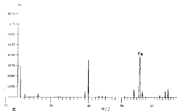
Figure 1. Partial mass spectra from various samples probed by LAMMA. Positive ion spectra show major peaks identified by their mass to charge ratios ( m/z ) where they are assumed to have a unit positive charge. Ordinate gives peak height rather than integrated peak intensity. Na 23; Mg 24; Al 27; P 30; S 32; K 39; Ca 40; Fe 56; Cu 63. (a) Cytoplasm of a Gaucher cell showing a high iron-related peak ( m/z = 56 ). (b) Genetic haemochromatosis, prior to phlebotomies; siderosomes in hepatocytes. (c) Same sample as (b), but the probed cell was a Kupffer cell; note that the iron-related peak is much lower than that of hepatocytic siderosomes. (d) Thalassaemia major, liver biopsy of a 3 month old infant showing an extremely high iron signal (saturated peak), as well as a significant aluminium peak ( m/z = 27 ). (e) Wilson's disease, patient 1. Probing of connective tissue cells from the pre-transplant cirrhotic liver show prominent copper ( m/z = 63 ) and iron ( m/z = 56 ) peaks.
